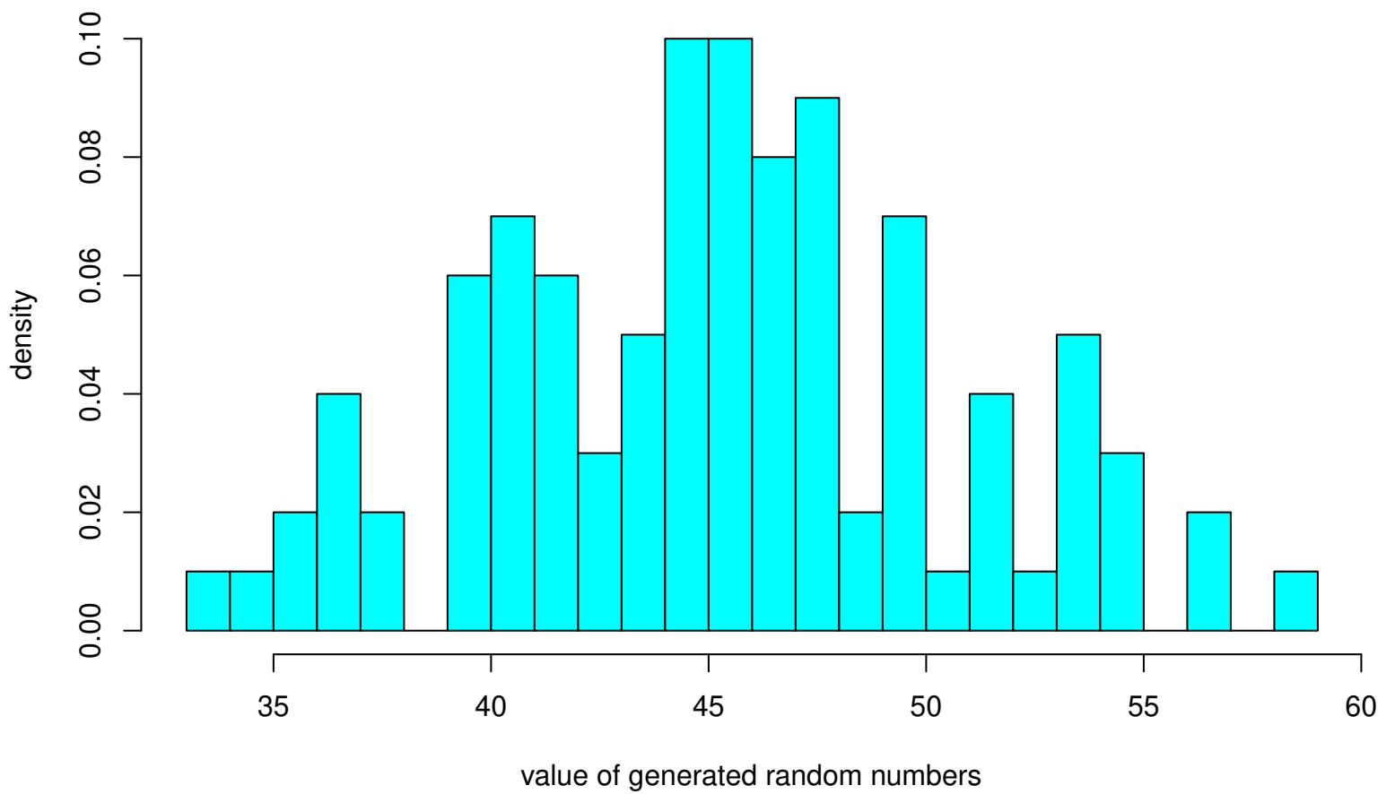
Histogram of Generated Random Numbers
