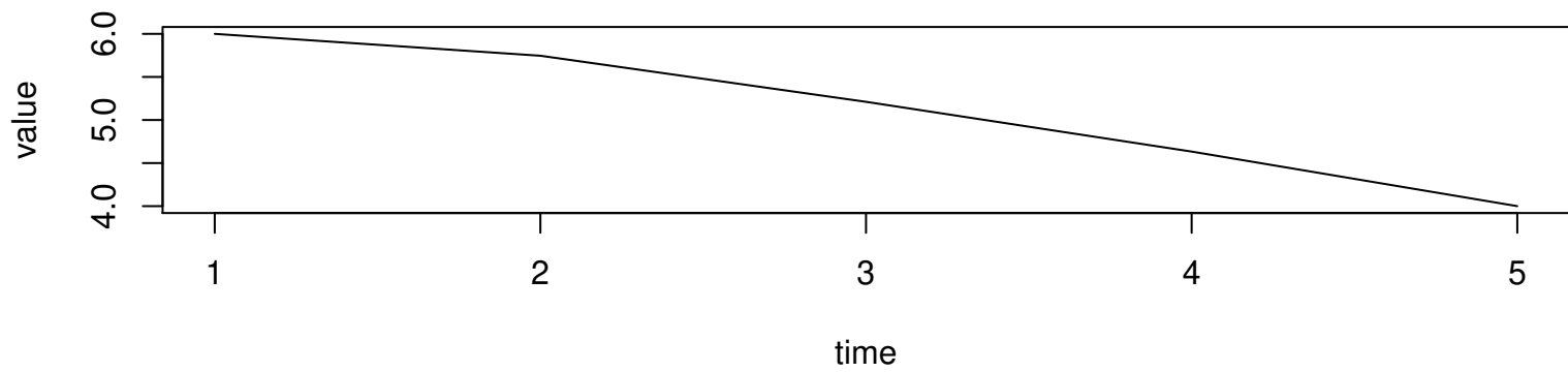
Working Time Series ( \lambda=0.5 , d=0 , D=0 )
