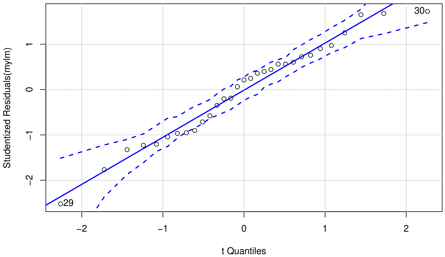
QQ Plot
