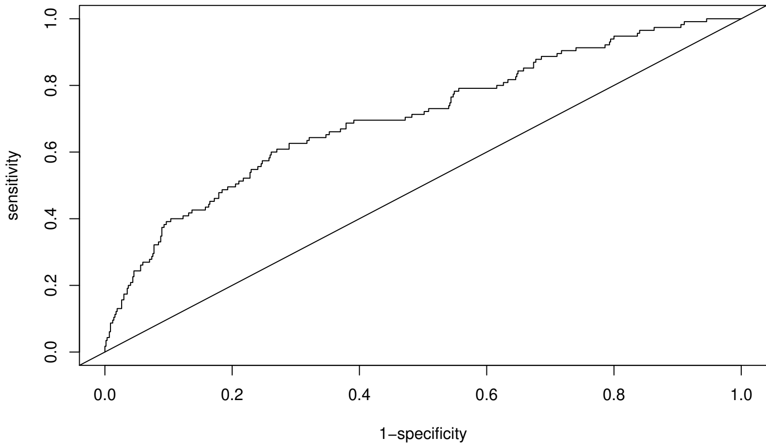
ROC plot
