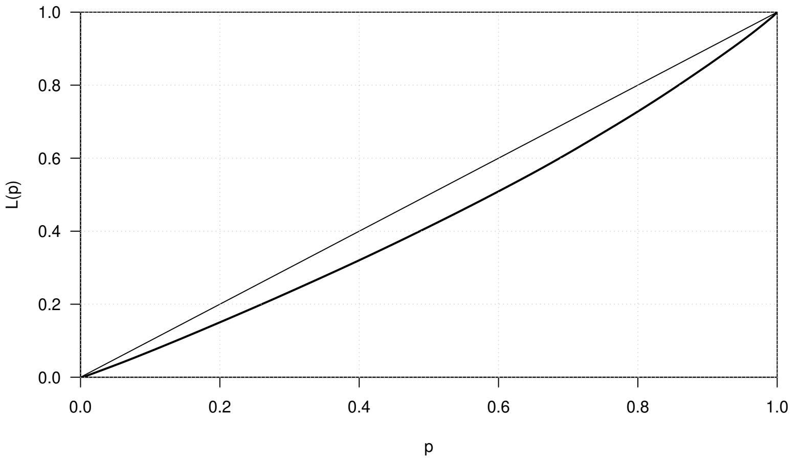
Lorenz curve
