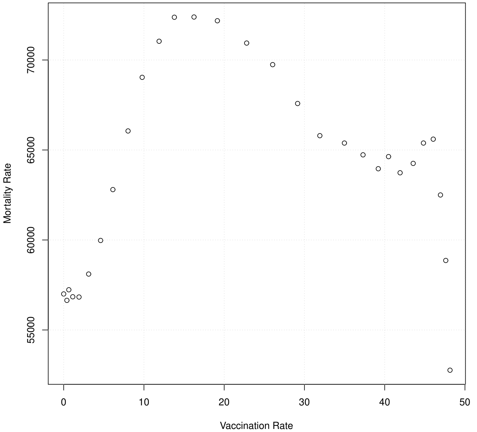
Scatterplot
