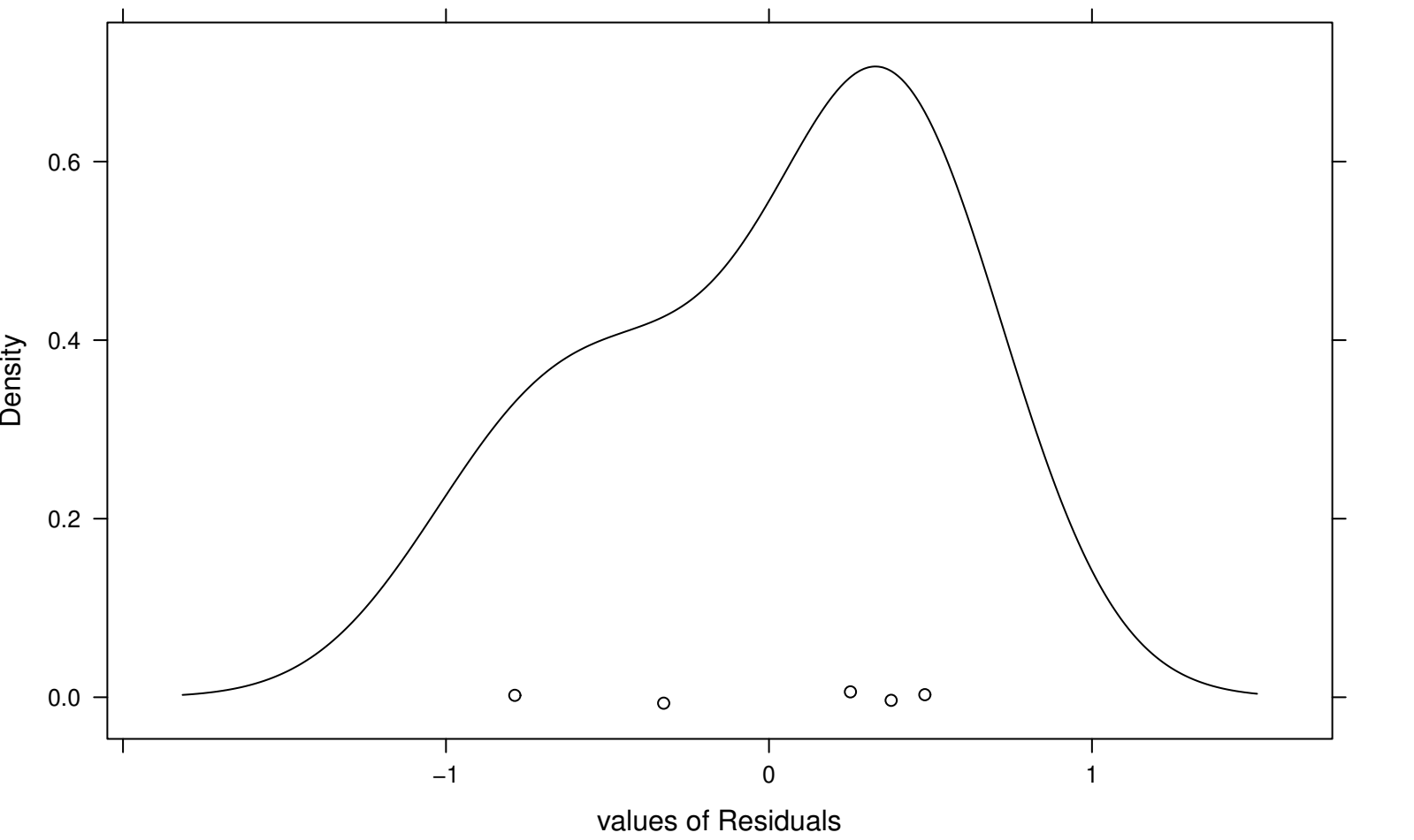
Residual Density Plot
